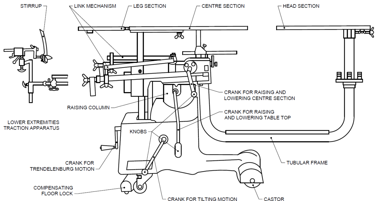
Fig. 1 ALBEE'S TYPE ORTHOPAEDIC OPERATION TABLE
